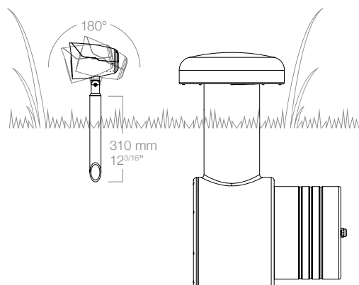
CLG-W12 below ground garden installation. On patios or decks install within a suitably sized planter.
